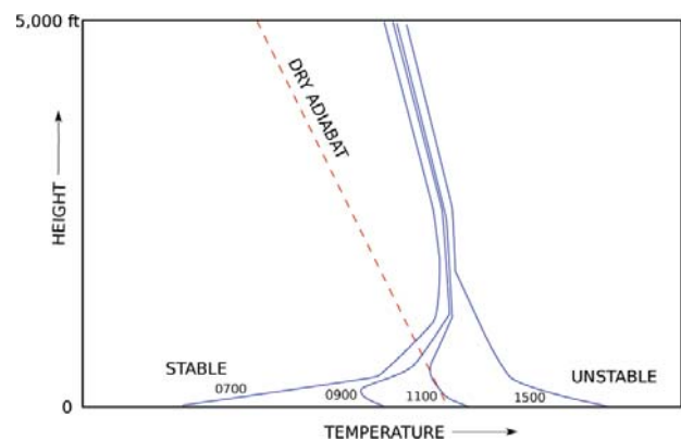
Change in temperature structure between 0700 and 1500. Strong surface inversion at 0700 is eroded throughout the day by surface heating producing an unstable layer at the surface.
