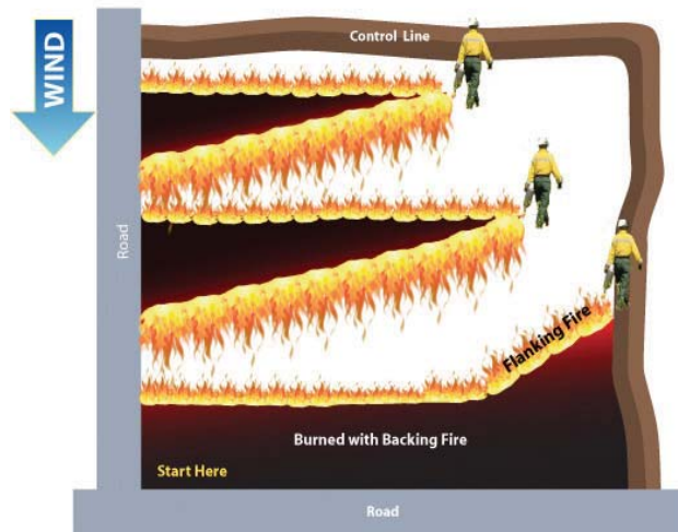
Strip-heading fire technique.
