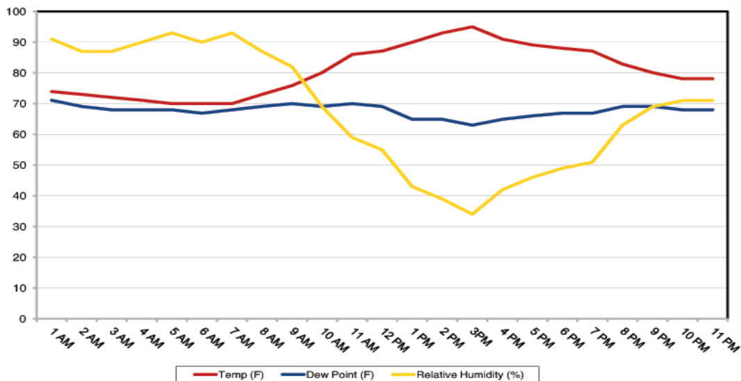
Daily cycle of temperature and relative humidity.
