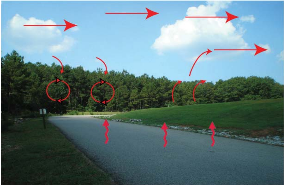
Convections and eddies for open areas.
