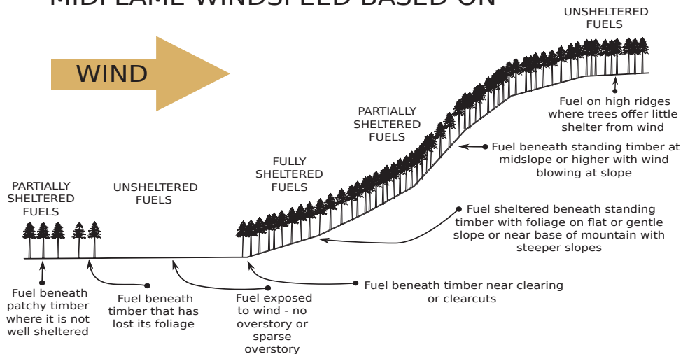
How slope position and canopy closure influence wind speed.
