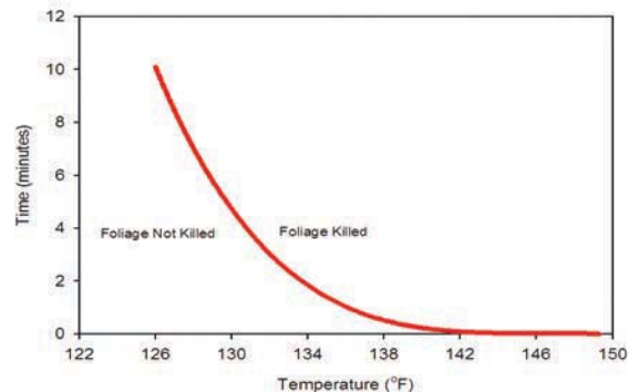
Lethal time-temperature curve.
