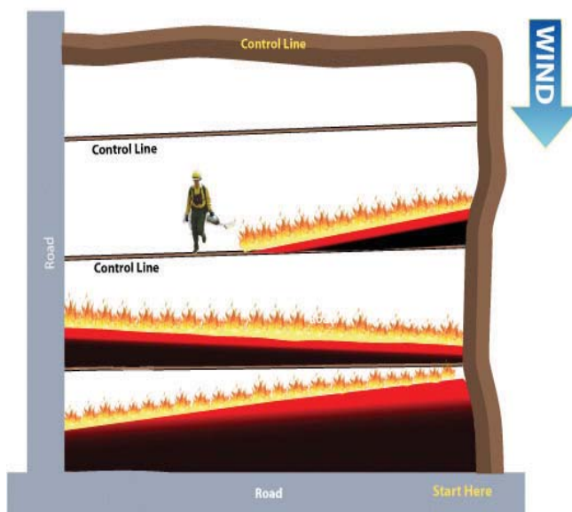
Backing fire technique.
