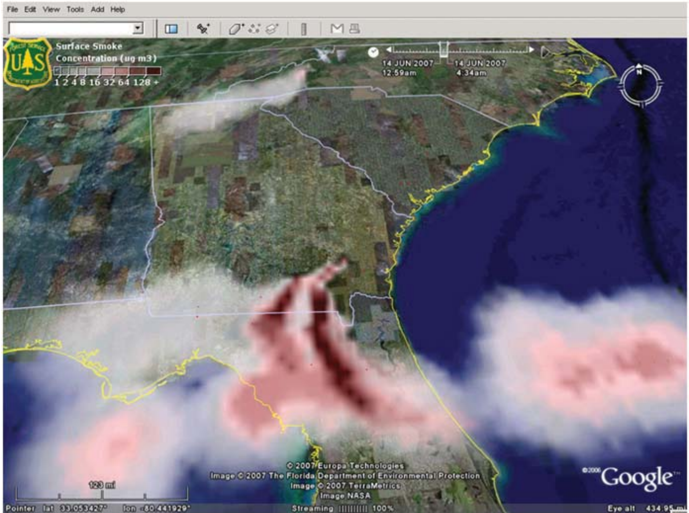
Sample output from Bluesky showing surface PM 2.5 concentrations.
