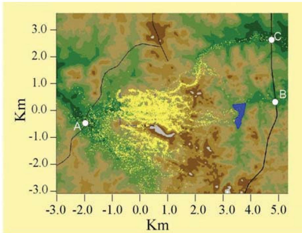
Sample output from PB-Piedmont showing smoke (yellow particles) moving down drainages and crossing roads at points A, B, and C.
