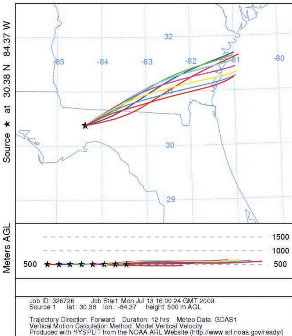
Hysplit trajectories showing possible plume paths over a 12 hour period.
