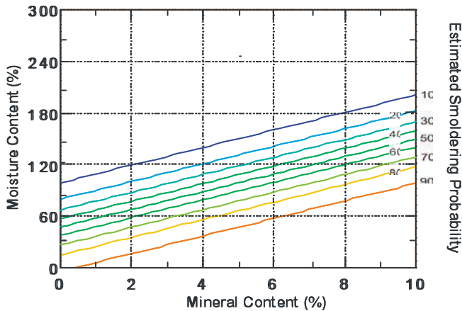
Estimated Smoldering Potential (ESP) of root mat soils expressed as a percent based on soil moisture and mineral content.
