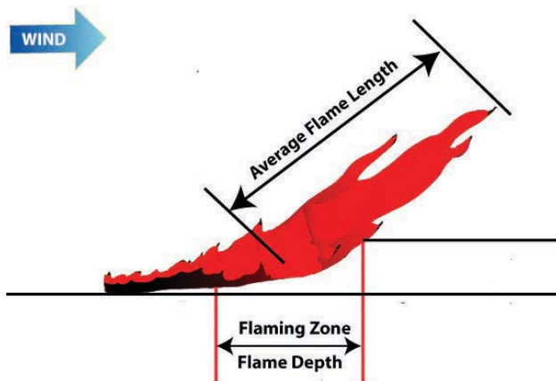
Flame dimensions for a wind driven fire.
