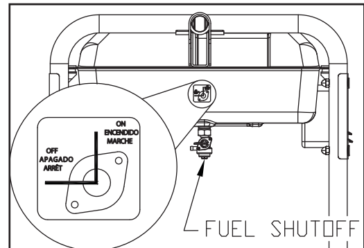
Figure 13 - Engine ON/OFF Switch
